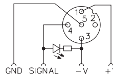
(PNP LED Version) Isolated Power Supply
