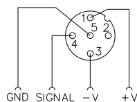
(No LED Version) Isolated Power Supply
