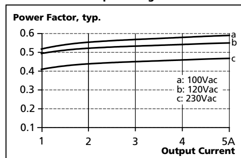
Fig. 3-4 Power factor vs. output load at 12V output voltage
